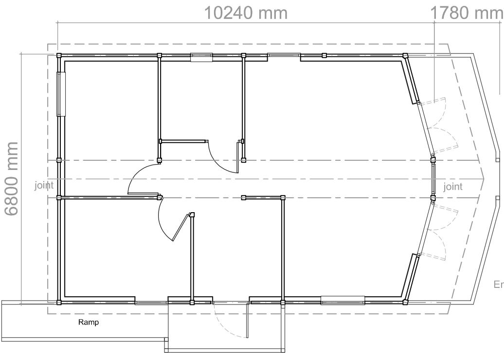
Floor Plan
