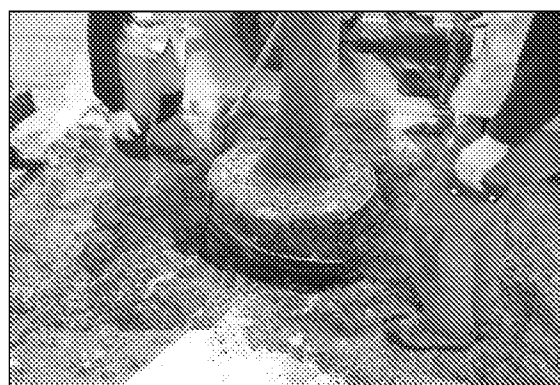
Photo 58: This excavated tree shows the root deflectors that were installed when it was planted seven years previously. The product has deflected roots downwards and prevented damage to the adjacent surfacing. Note that this is a permeable sandy soil and the roots were able to grow beneath the bottom of the deflectors.
