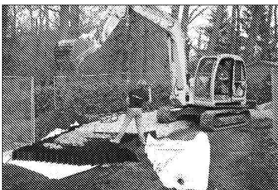
Photo 11: Cellular products are a very effective means of providing ground protection where heavy vehicle use is expected. Here, it is being used to temporarily widen an existing road, to be removed once the construction is finished.
