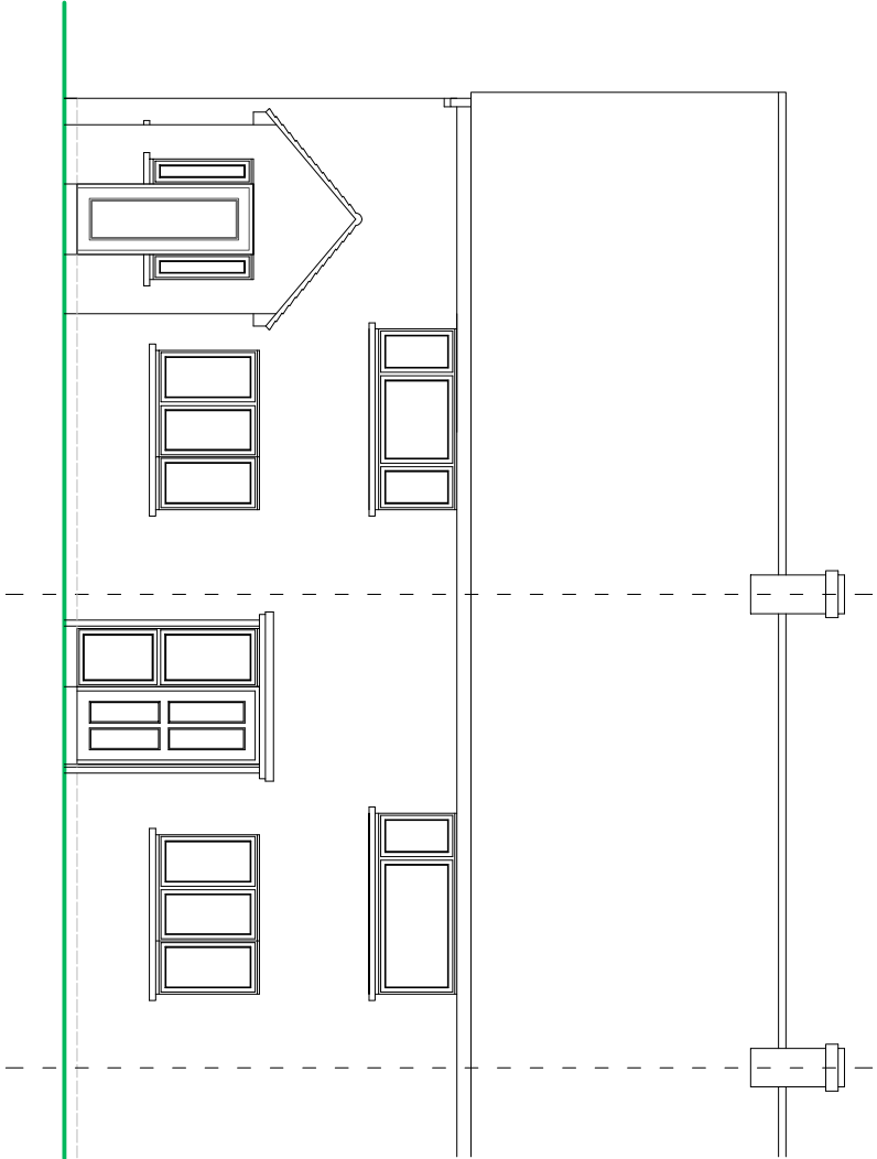
FRONT ELEVATION
