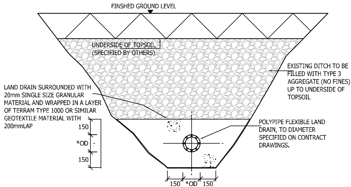
LAND DRAIN IN EXISTING DITCH
