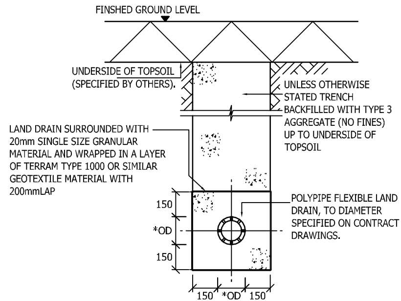
LAND DRAIN
