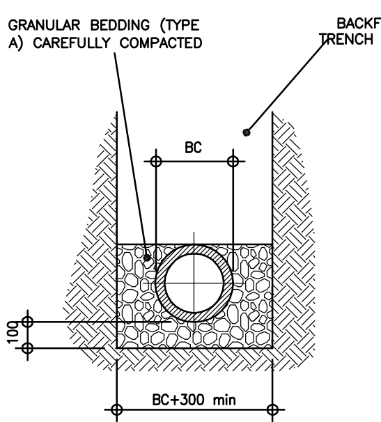
GRANULAR SIDE FILL TO BE USED WHERE COVER TO CROWN OF PIPE IS GREATER THAN 900mm UNDER ROADS, FOOTWAYS & HARDSTANDINGS
