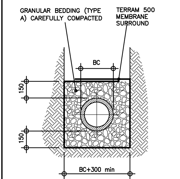
GRANULAR SURROUND TO BE USED WHERE PIPE PASSES WITHIN 3M OF NEW OR EXISTING TREES UNLESS PIPE REQUIRED CONCRETE SURROUND
