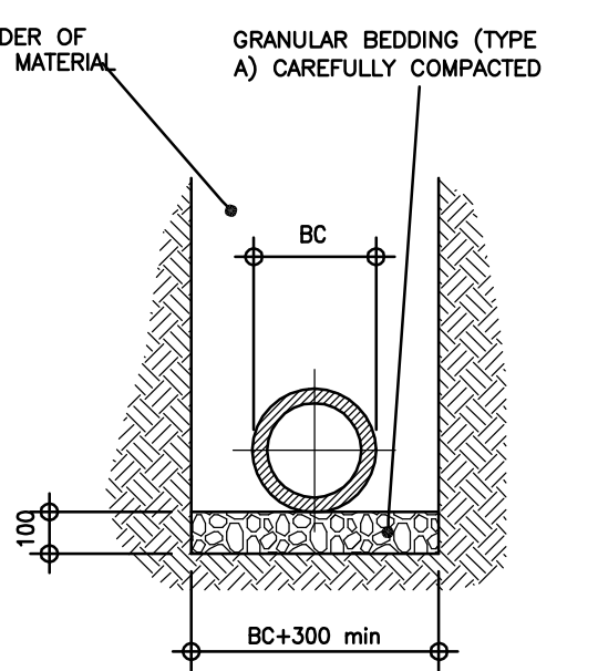
GRANULAR BED TO BE USED WHERE COVER TO CROWN OF PIPE IS GREATER THAN 600mm IN LANDSCAPED AREAS
