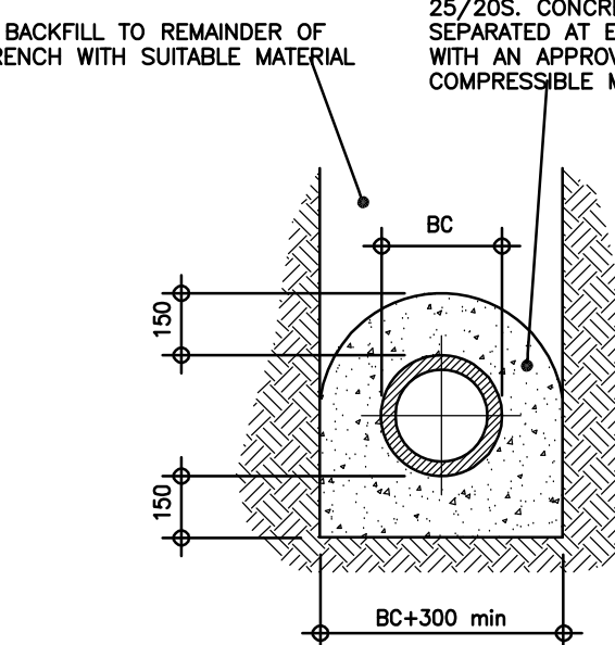
CONCRETE SURROUND
