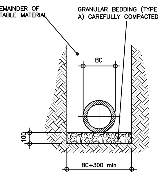
GRANULAR BED
