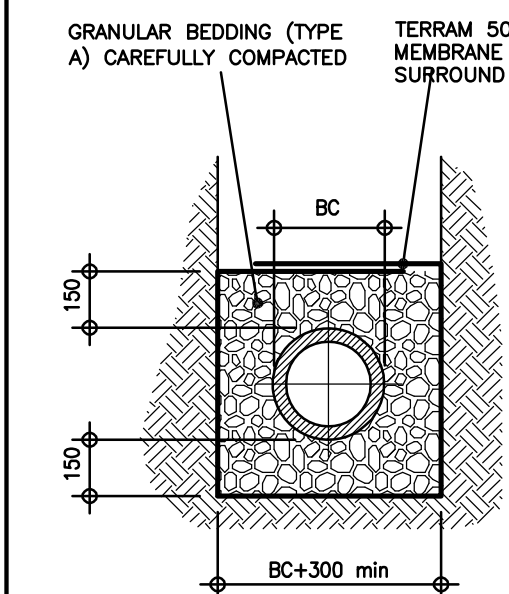
GRANULAR SURROUND
