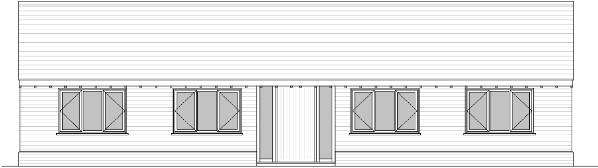
Approved West Elevation
