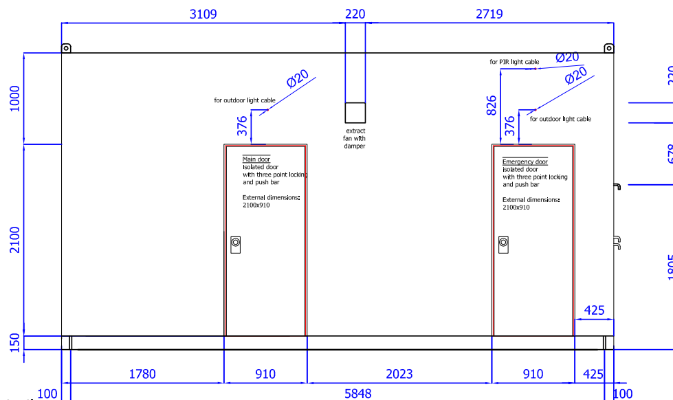
B-B view
