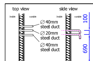
Detail 1 - SCADA antenna cable entry
