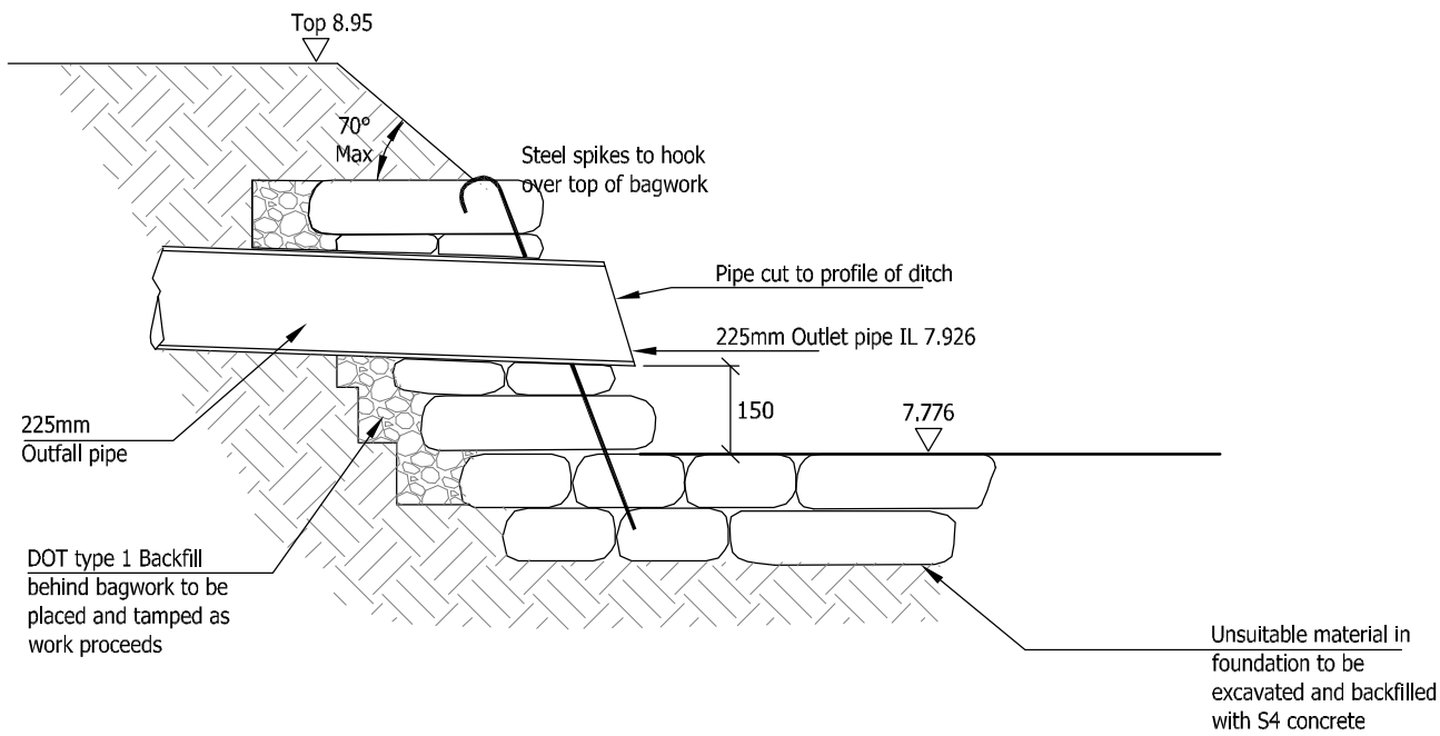
225mm DIA OUTFALL FROM POND TO SOUTHERN DITCH - HEADWALL SECTION
