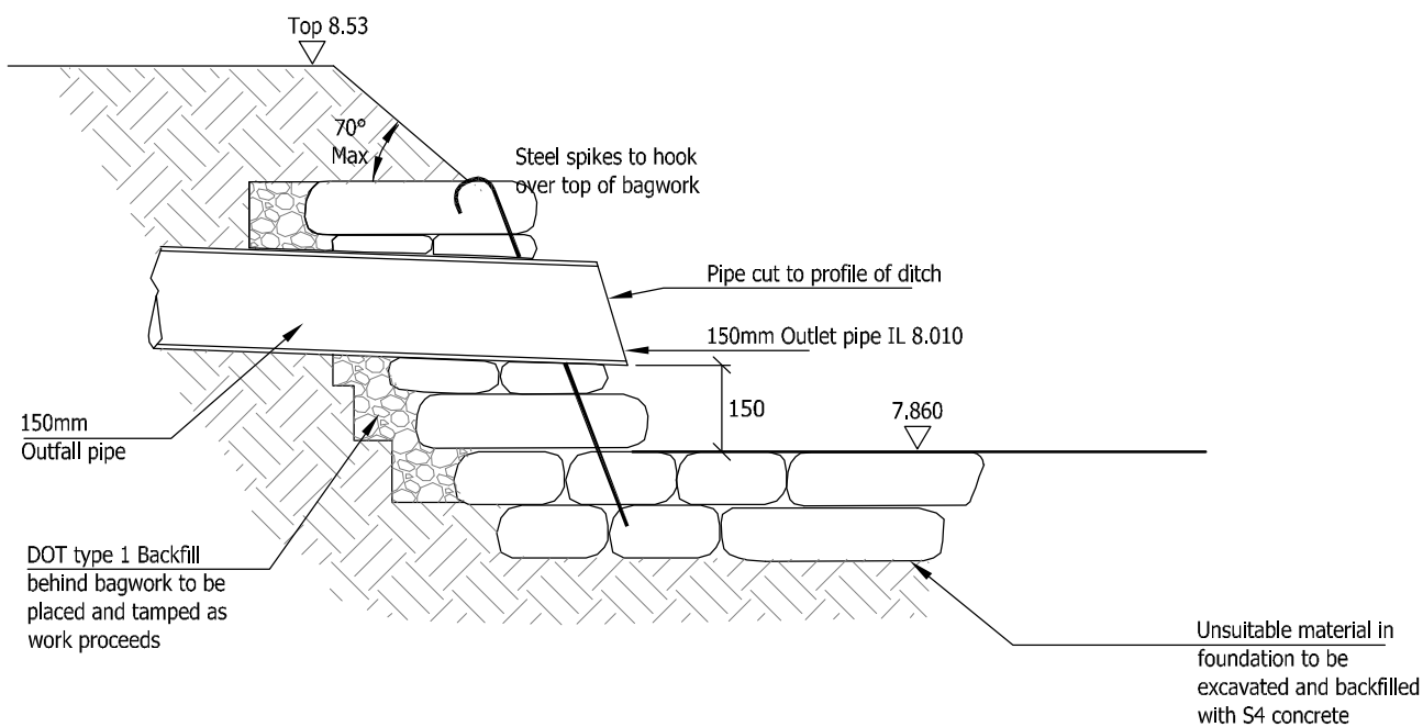
150mm DIA OUTFALL FROM LAND DRAIN TO EASTERN DITCH - HEADWALL SECTION
