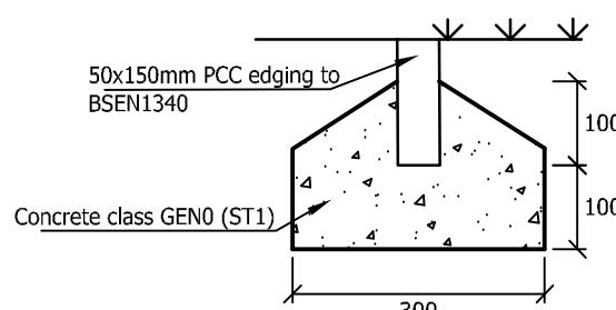
PCC EDGING KERB As denoted by
