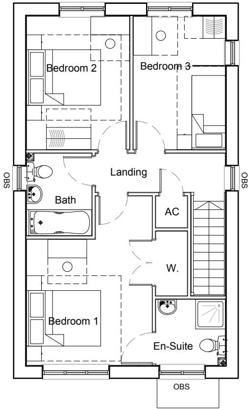
First Floor Plan *Obs - Obscured Glass
