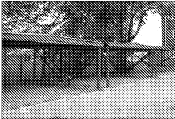
Photo 34: These carports are formed by wooden posts above a three dimensional cellular no-dig and load-spreading surface of permeable crushed stone.
