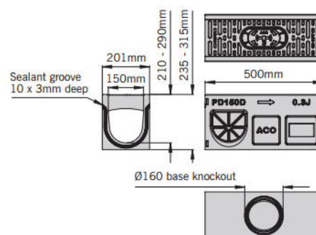
PD150D access unit
