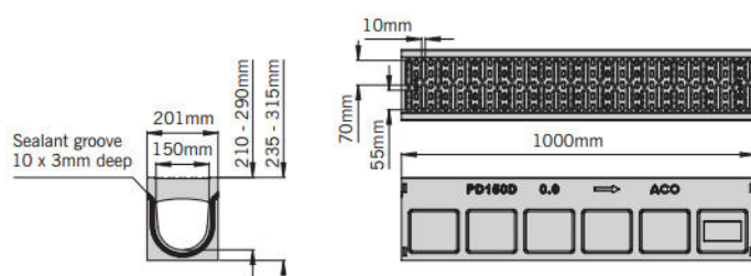
PD150D constant depth channel
