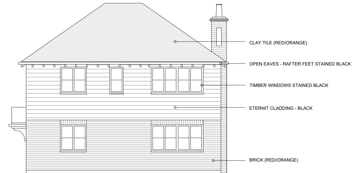
side/south
