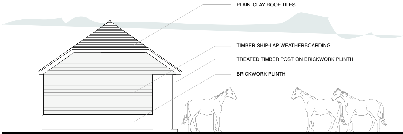
Proposed North West Elevation at 1:100 scale
