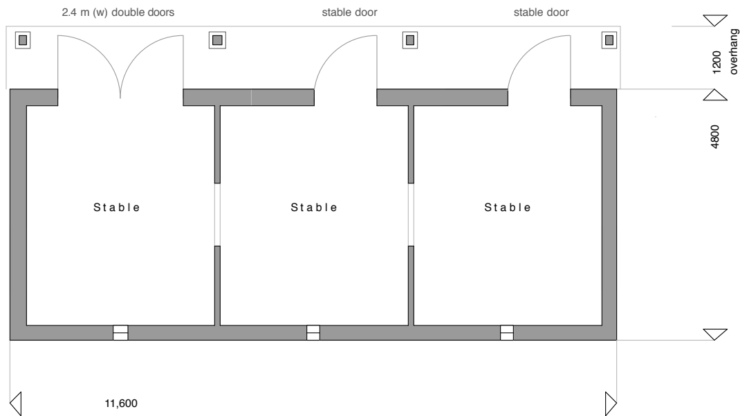
Proposed Ground Floor Plan at 1:100 scale
