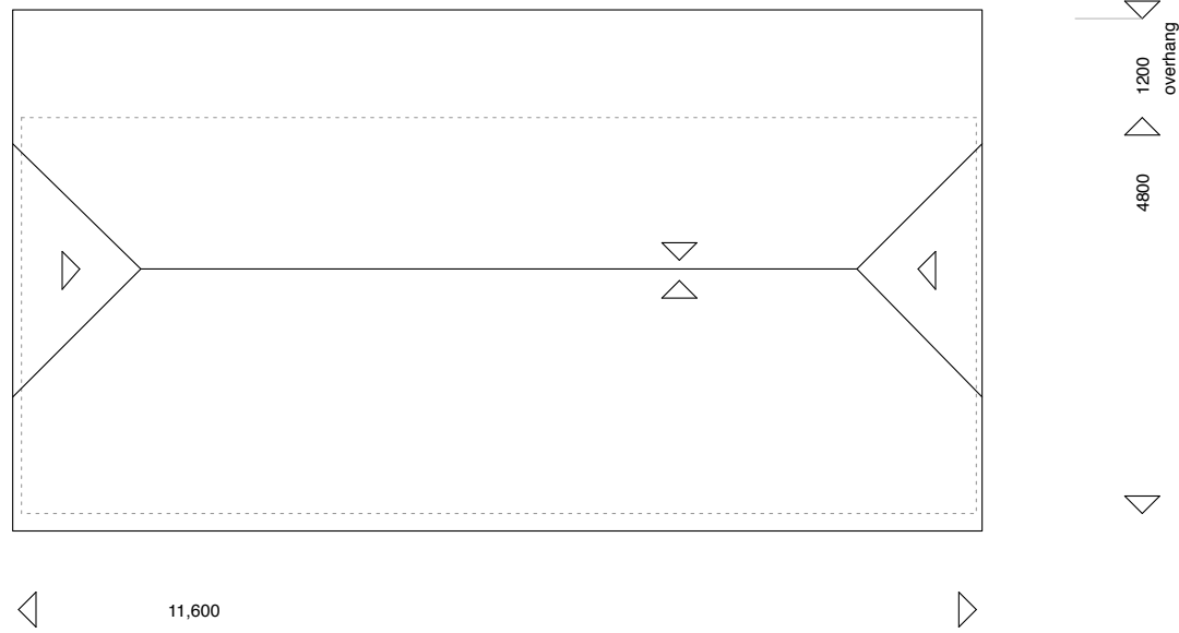
Proposed Roof Plan at 1:100 scale
