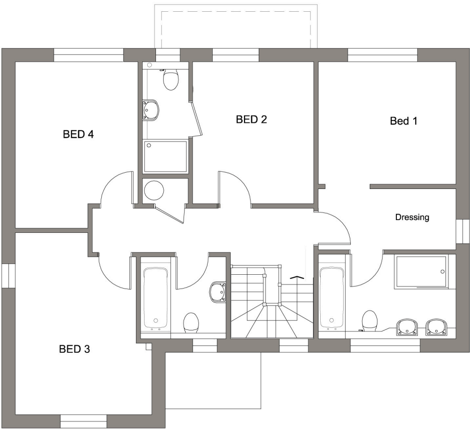
FIRST FLOOR PLAN PLOTS - 1, 4 & 5
