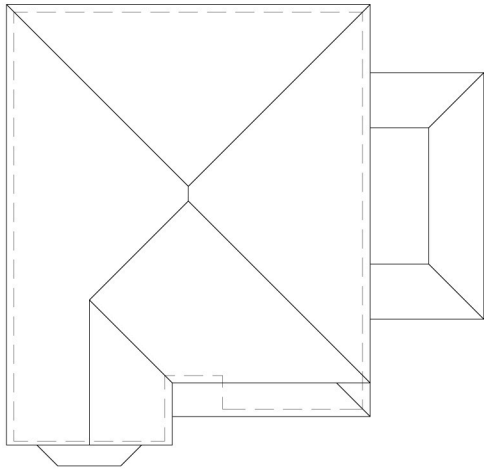
ROOF PLAN SCALE 1-200 PLOT 2(handed) & PLOT 3
