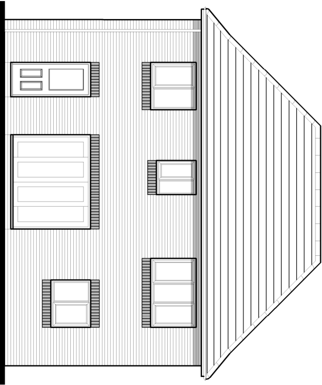
Rear Elevation
