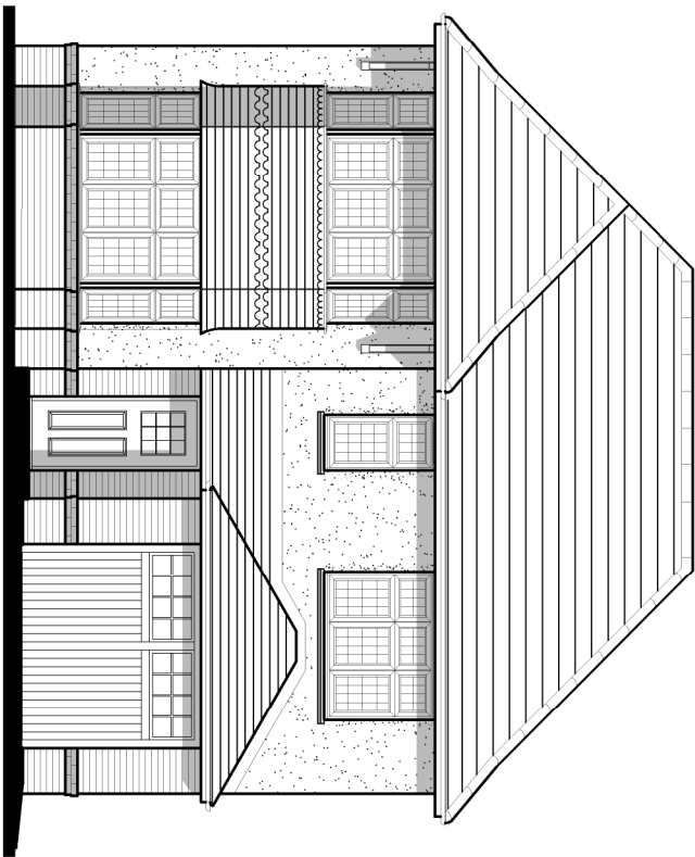
Front Elevation
