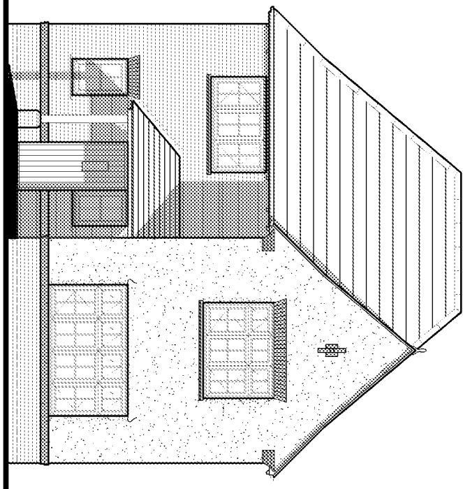
Front Elevation
