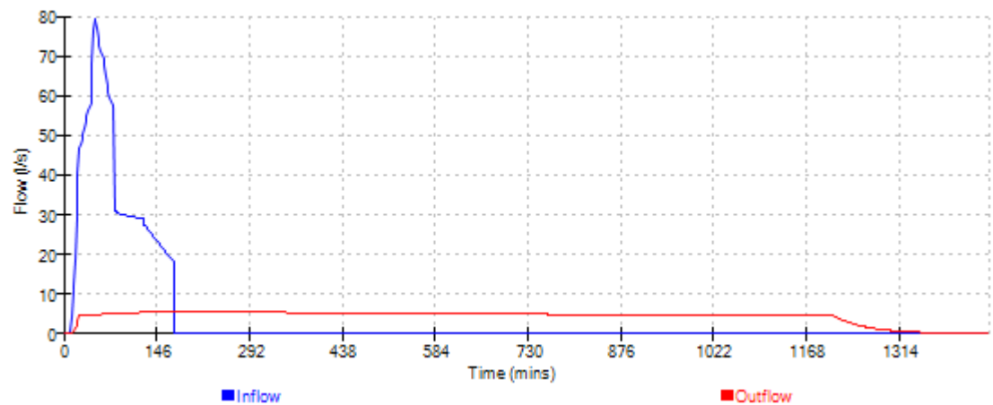
Cascade Event: 60 min Winter for 15104 Soakaway cascade Rev C.SRCX
