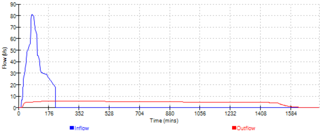
Cascade Event: 120 min Winter for 15104 Soakaway cascade Rev C.SRCX
