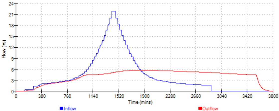
Cascade Event: 2880 min Summer for 15104 Soakaway cascade Rev C.SRCX
