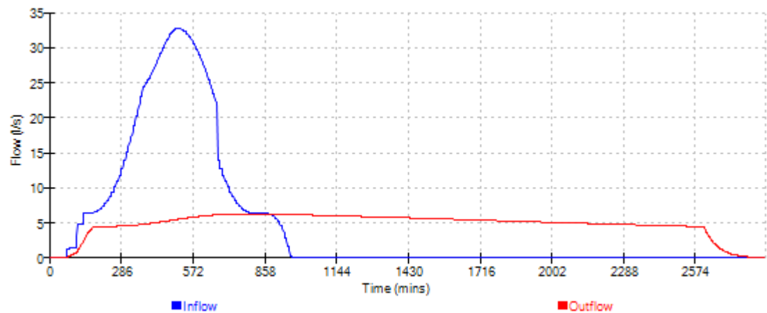
Cascade Event: 960 min Winter for 15104 Soakaway cascade Rev C.SRCX
