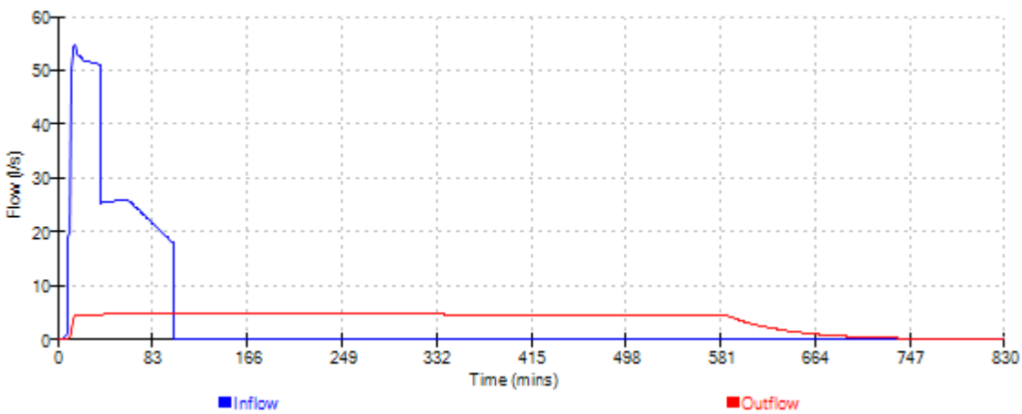
Cascade Event: 15 min Summer for 15104 Soakaway cascade Rev C.SRCX
