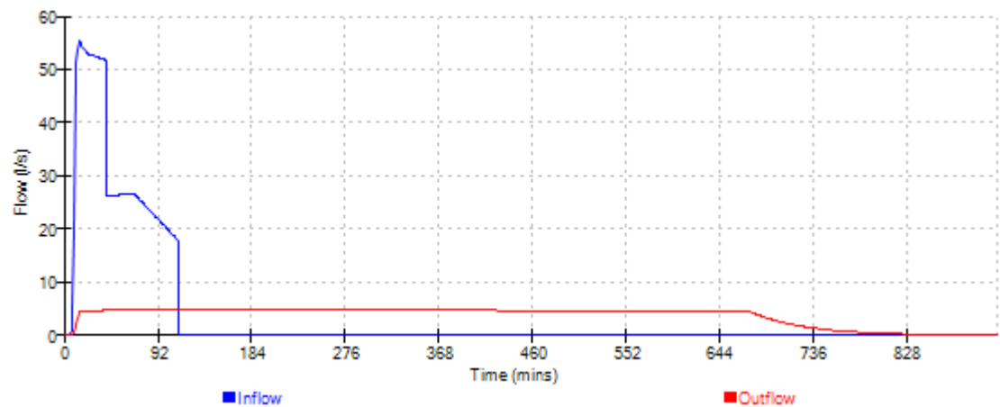
Cascade Event: 15 min Winter for 15104 Soakaway cascade Rev C.SRCX
