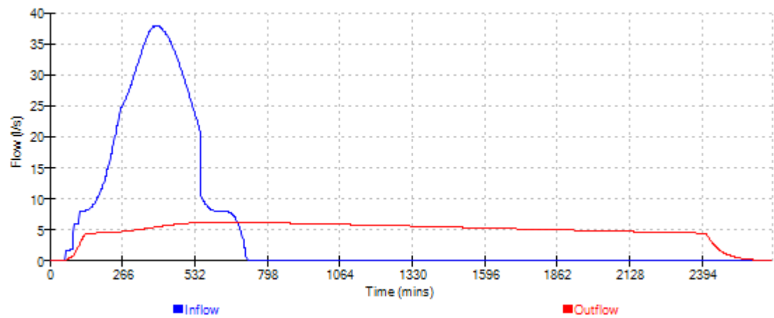
Cascade Event: 720 min Winter for 15104 Soakaway cascade Rev C.SRCX
