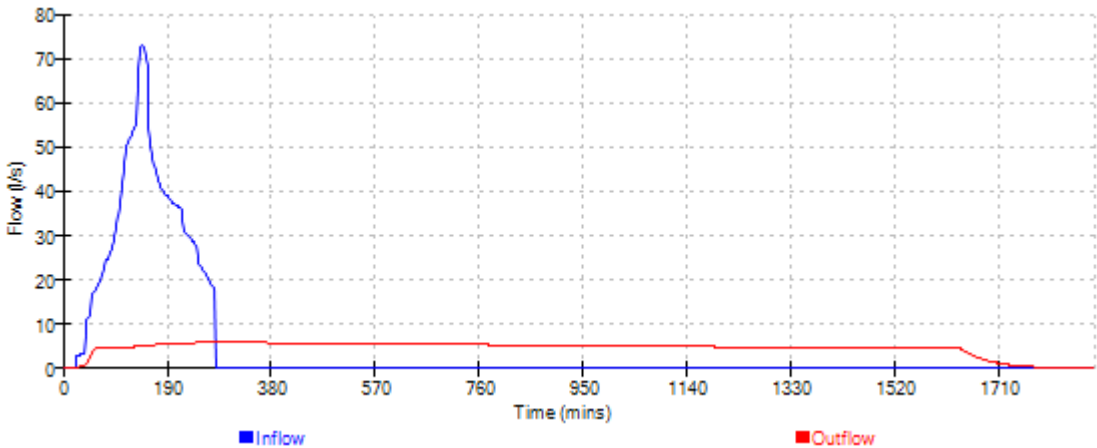
Cascade Event: 240 min Summer for 15104 Soakaway cascade Rev C.SRCX
