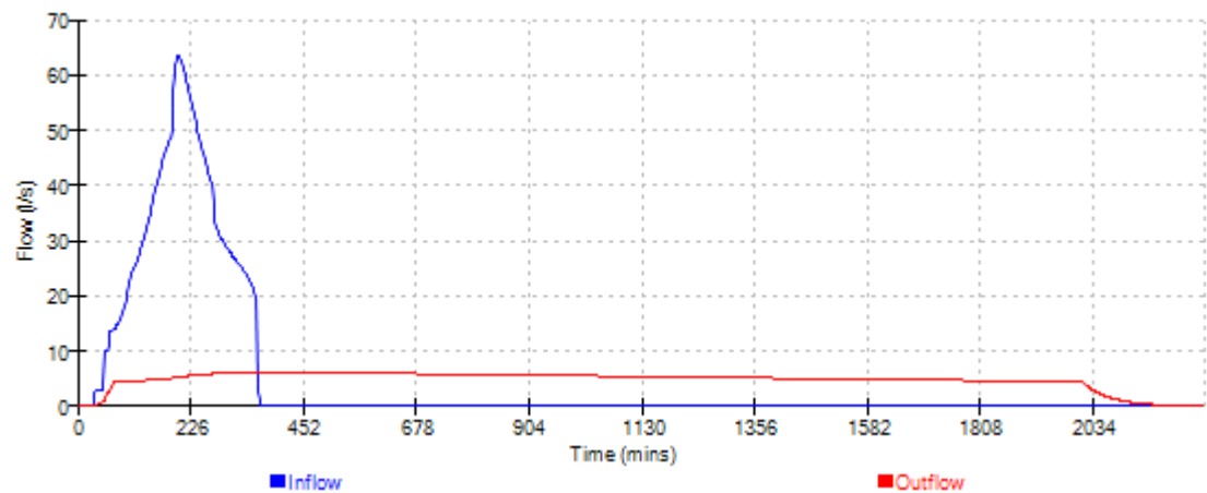
Cascade Event: 360 min Winter for 15104 Soakaway cascade Rev C.SRCX
