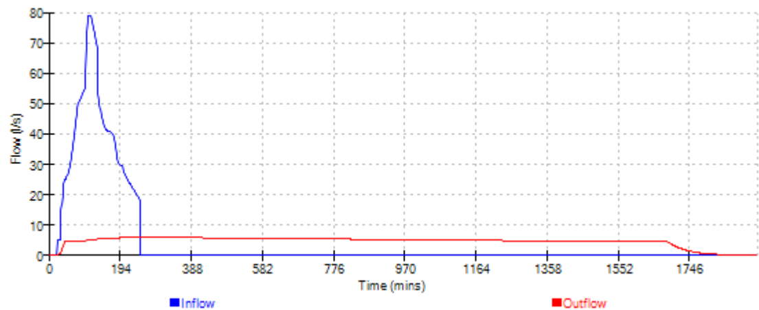
Cascade Event: 180 min Winter for 15104 Soakaway cascade Rev C.SRCX
