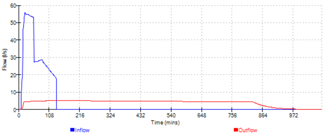
Cascade Event: 30 min Summer for 15104 Soakaway cascade Rev C.SRCX
