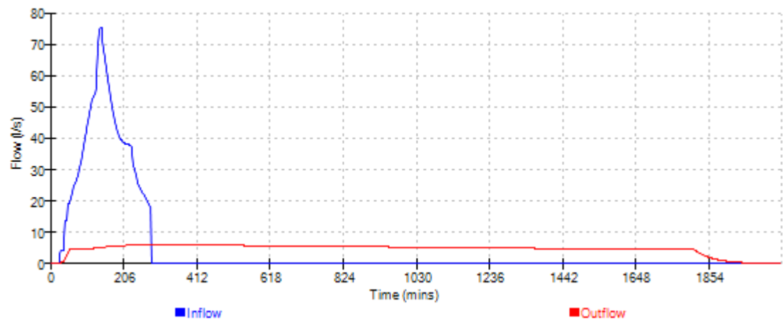
Cascade Event: 240 min Winter for 15104 Soakaway cascade Rev C.SRCX
