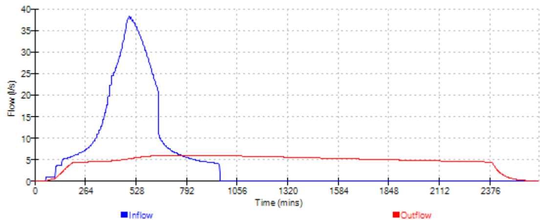
Cascade Event: 960 min Summer for 15104 Soakaway cascade Rev C.SRCX
