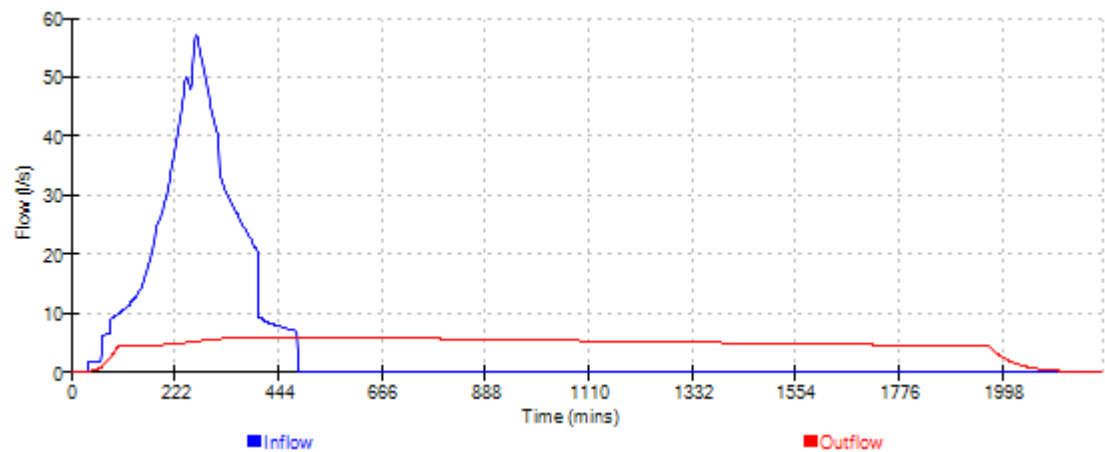
Cascade Event: 480 min Summer for 15104 Soakaway cascade Rev C.SRCX
