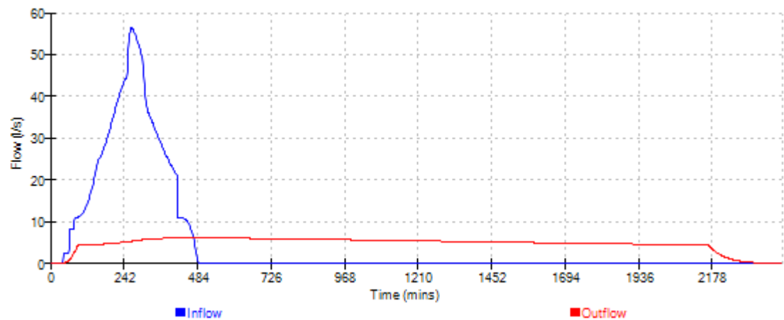
Cascade Event: 480 min Winter for 15104 Soakaway cascade Rev C.SRCX
