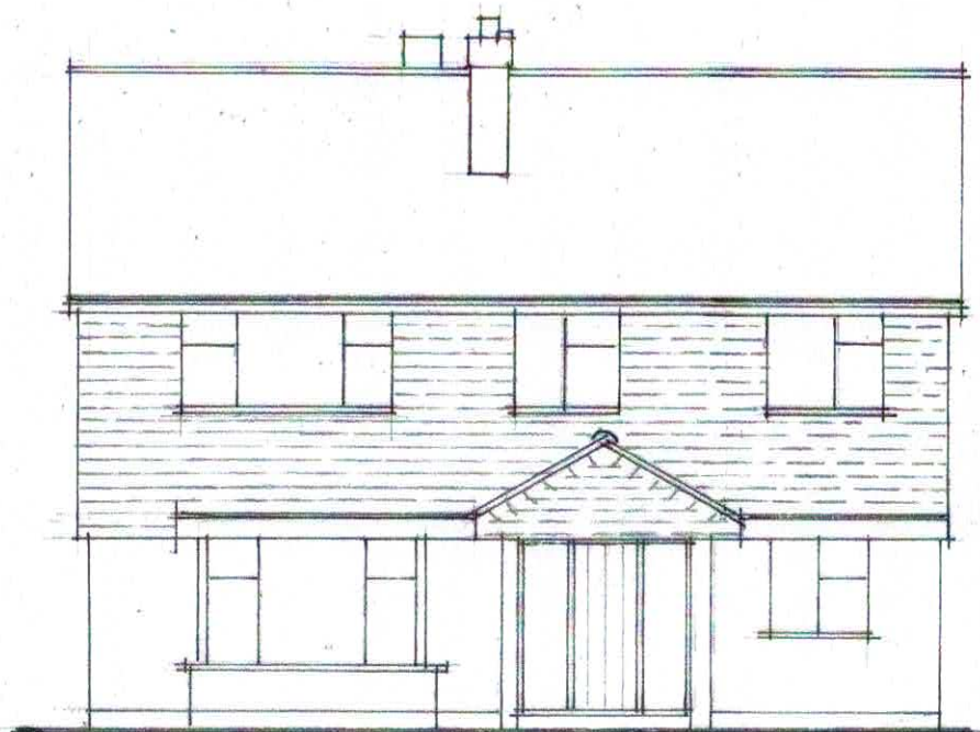
FRONT ELEVATION 1-100
