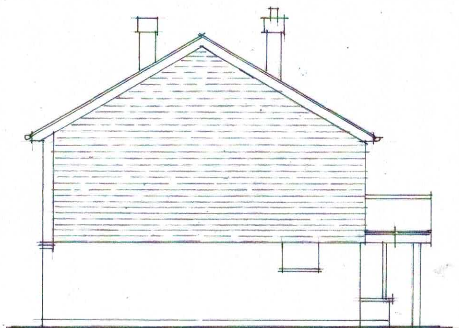
SIDE ELEVATION 1-100
