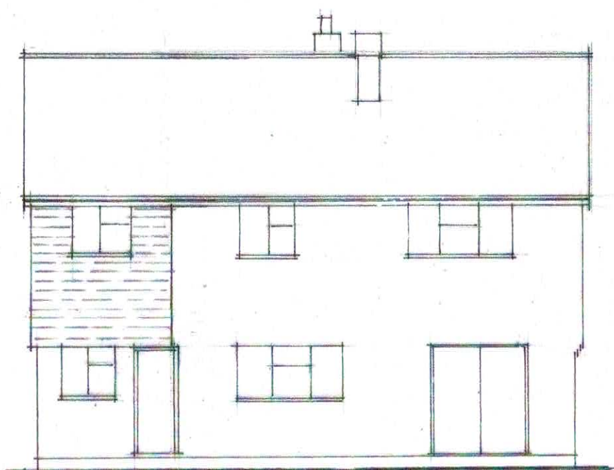
REAR ELEVATION 1-100
