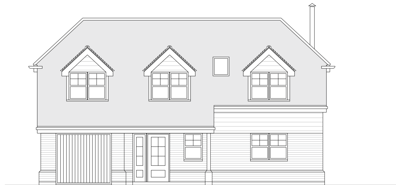
FRONT ELEVATION (SOUTH)
