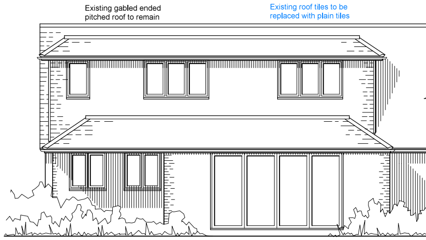
North Elevation
