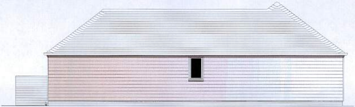
South Elevation 1:100
