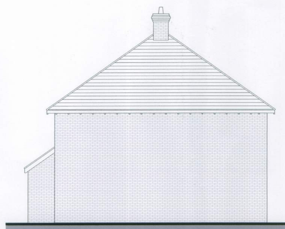
Elevation C
