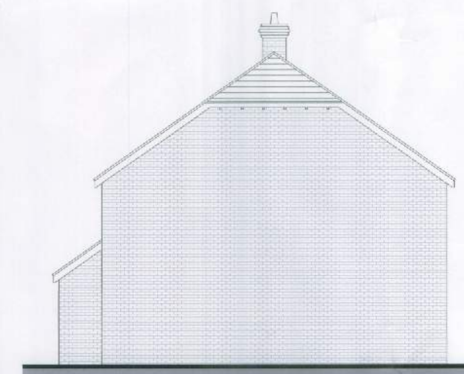
Elevation C
