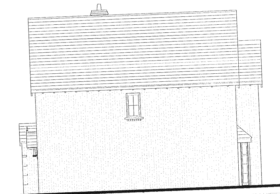
Elevation C
