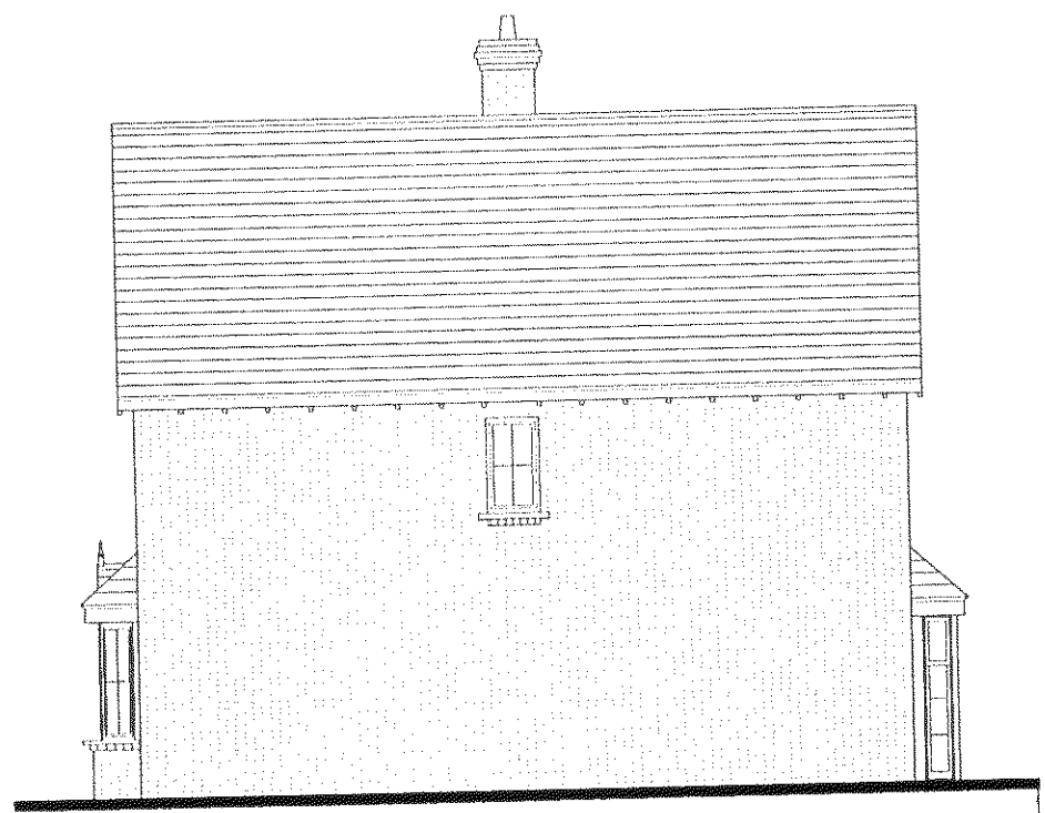
Elevation C
