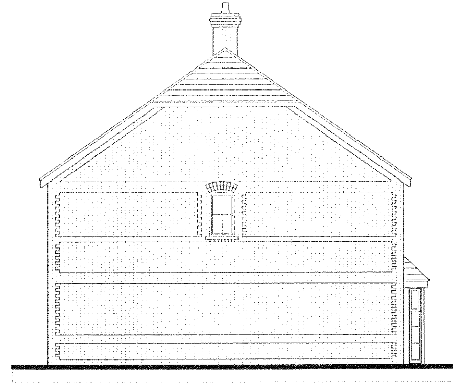
Elevation C
