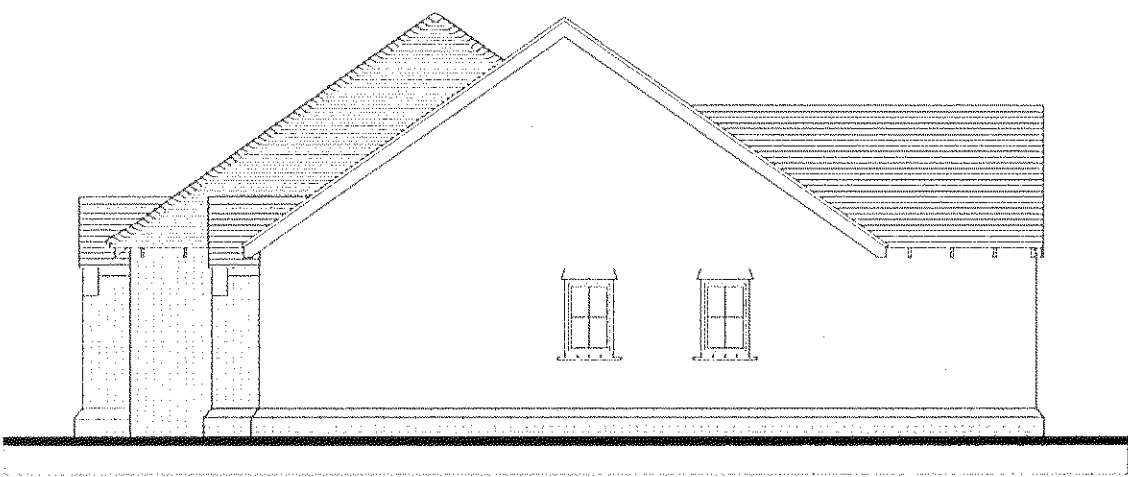
Elevation C
