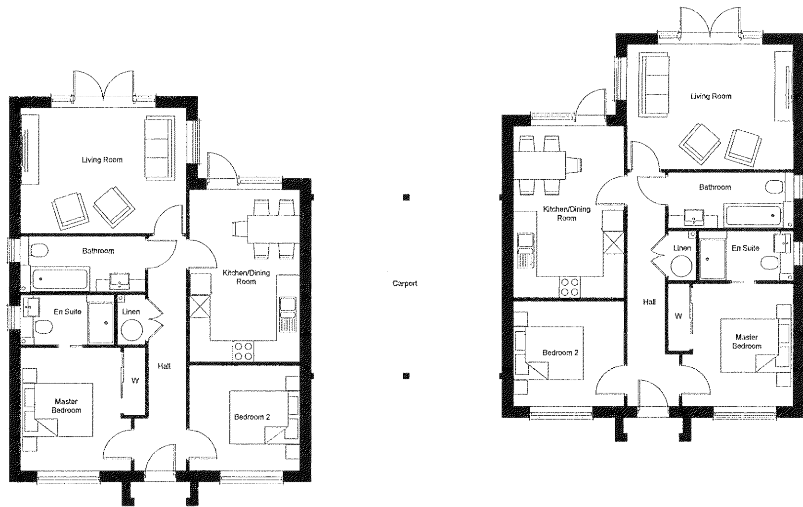
Floor Plan
