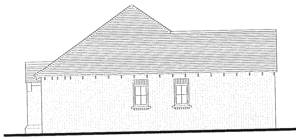
Elevation C
