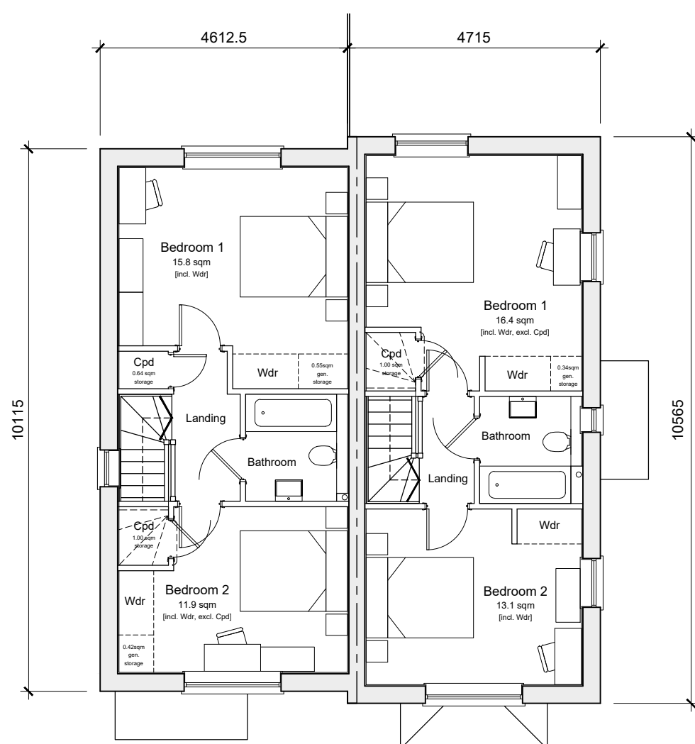
First Floor Plan Type A Plot B13 Type B Plot B12
