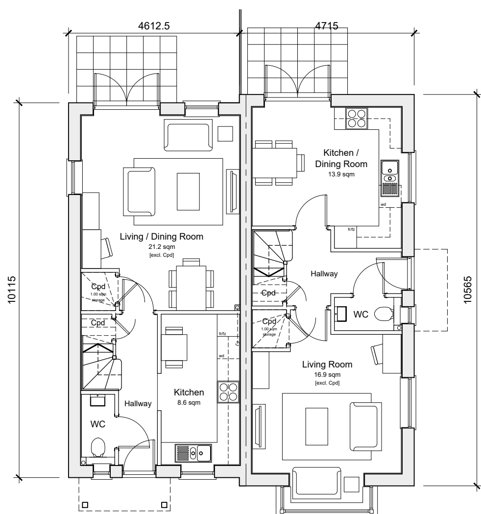
Ground Floor Plan Type A Plot B13 Type B Plot B12
