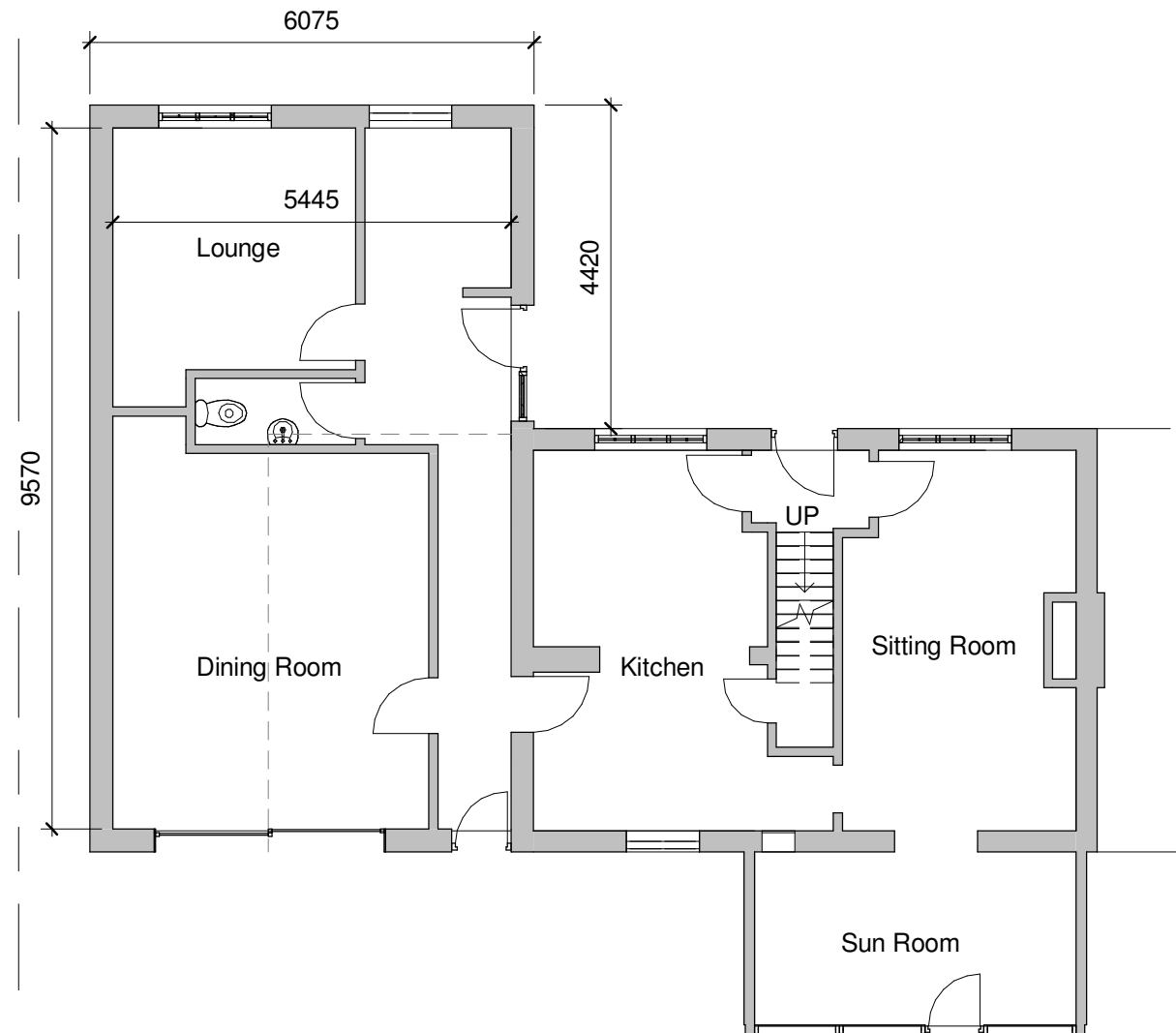
Proposed Ground Floor 1 : 100
