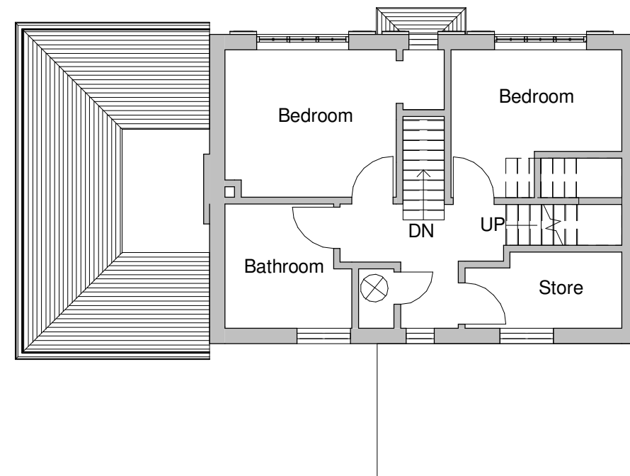
Existing First Floor 1 : 100
