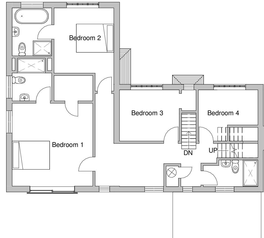
Proposed First Floor 1 : 100
