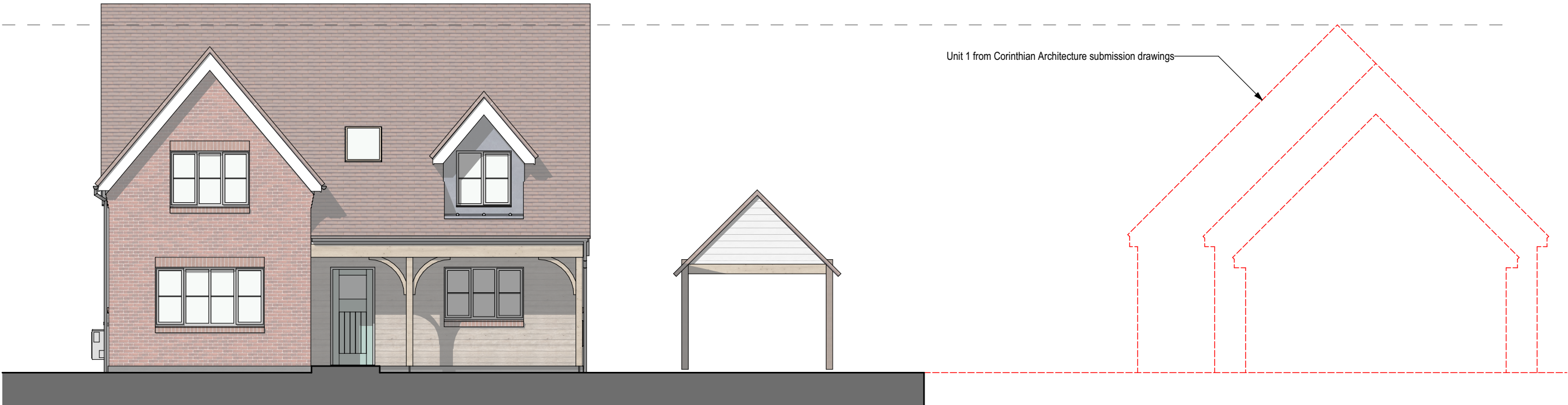
Front Elevation 1:100
