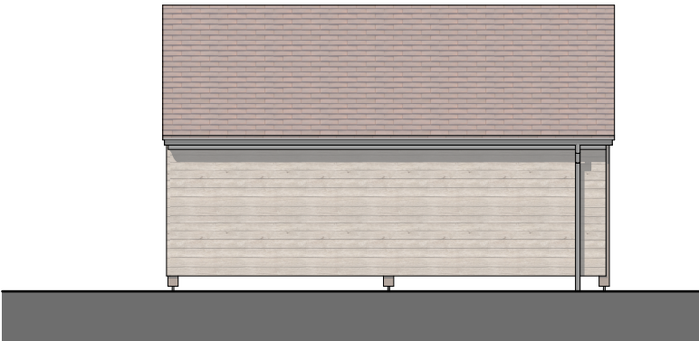
Side Elevation 1:100
