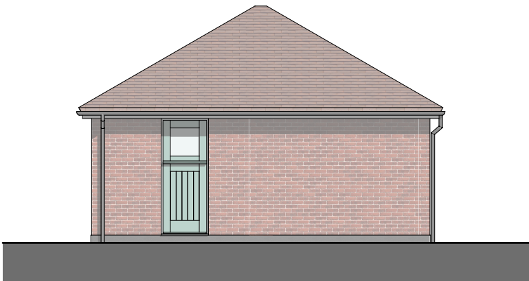
Side Elevation 1:100
