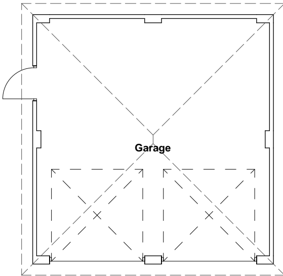
Ground Floor 1:100
