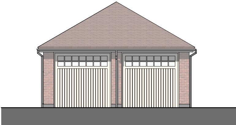
Front Elevation 1:100
