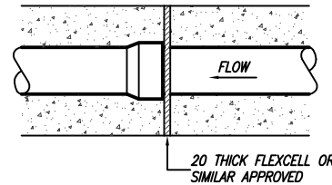
FLEXIBLE JOINT DETAIL FOR SOCKETED PIPES
