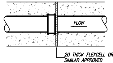
FLEXIBLE JOINT DETAIL FOR SLEEVED PIPES
