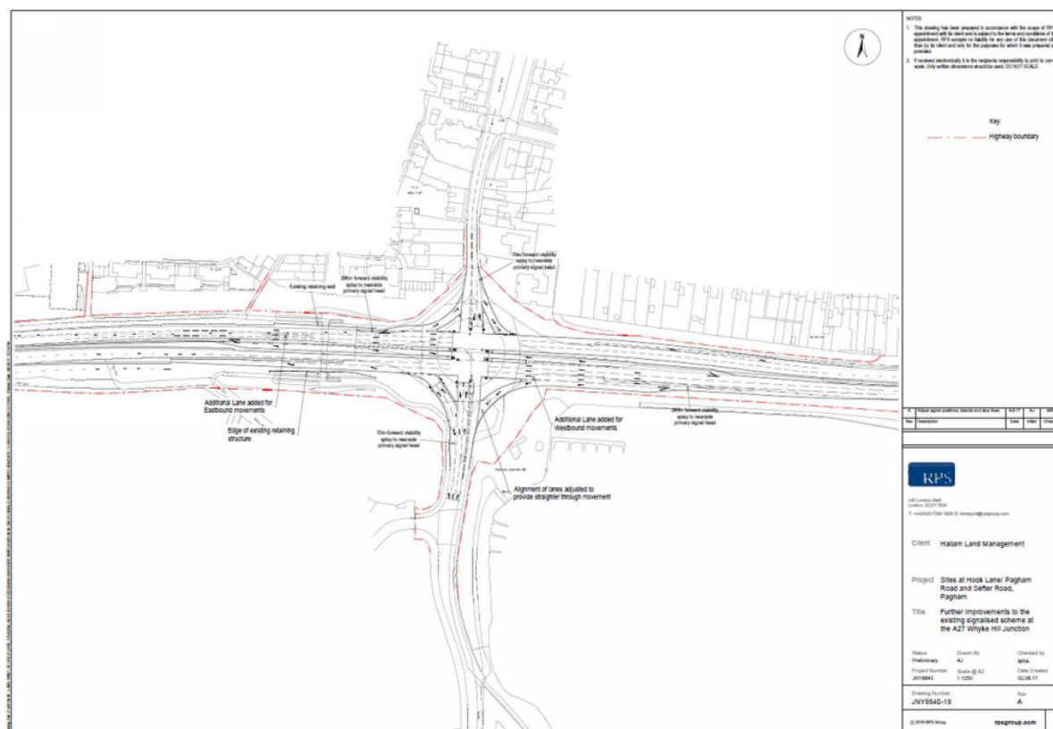
Figure 6.23: Whyke Roundabout mitigation scheme
