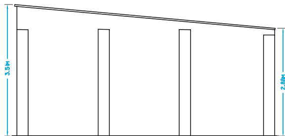
South Elevation
