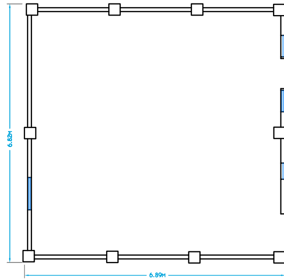
Ground Floor Floor Area 45.3m 2
