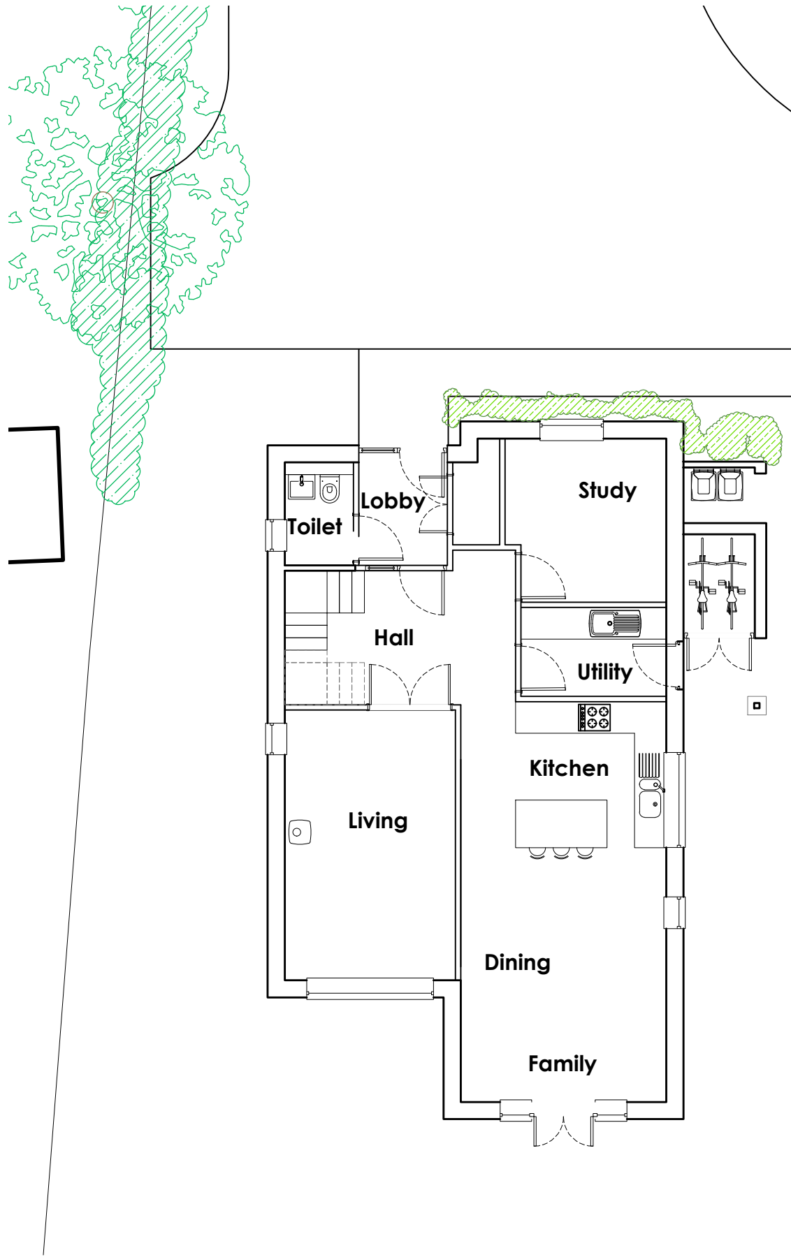
Ground & First floor plans 1:100 @ A3
