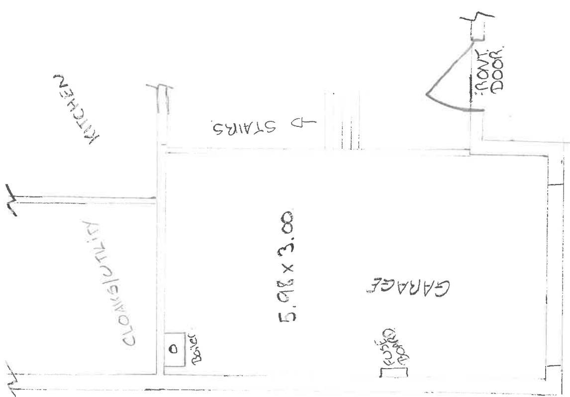
Existing Floor Plan (Garage area Only)
