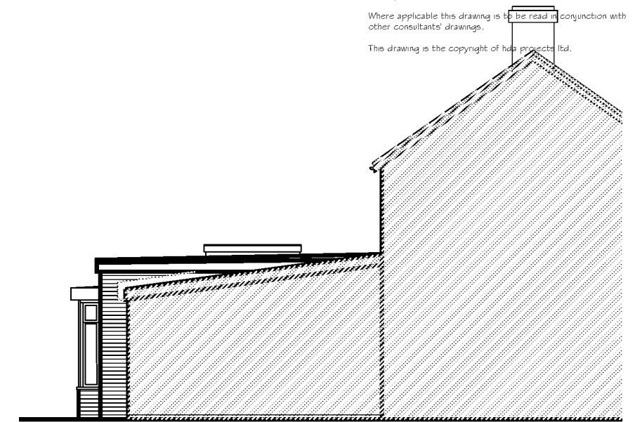
South Elevation
