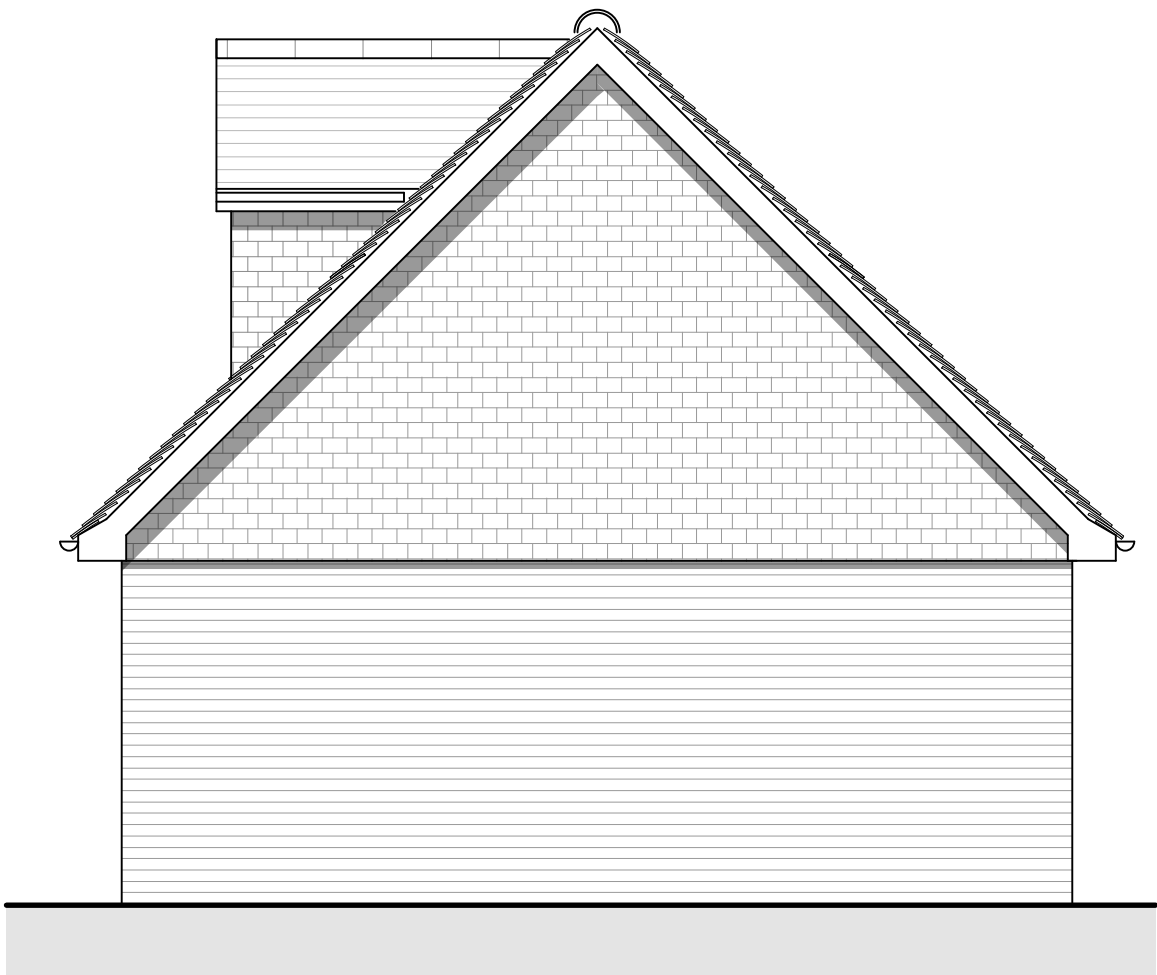
North-East Elevation Scale 1:50
