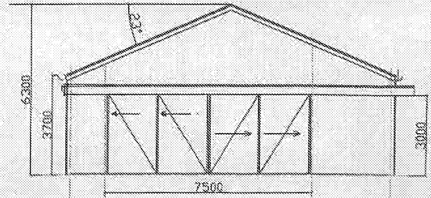
Double tracked sliding doors
