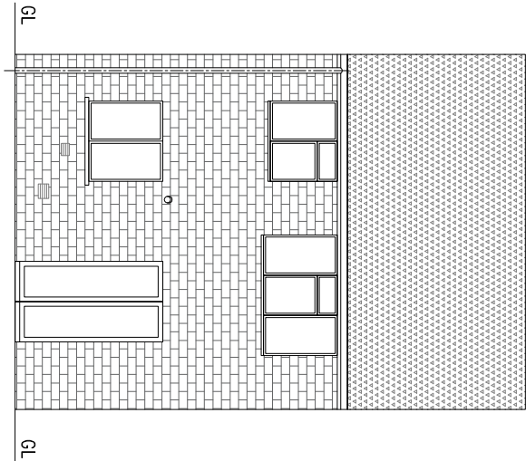
1 EXISTING REAR VIEW SCALE 1:100
