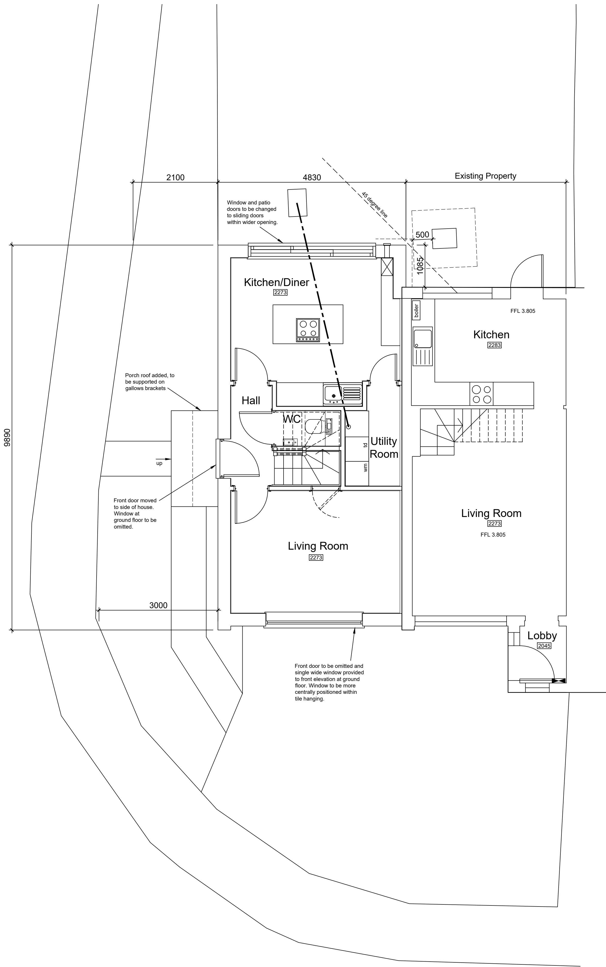
Ground Floor
