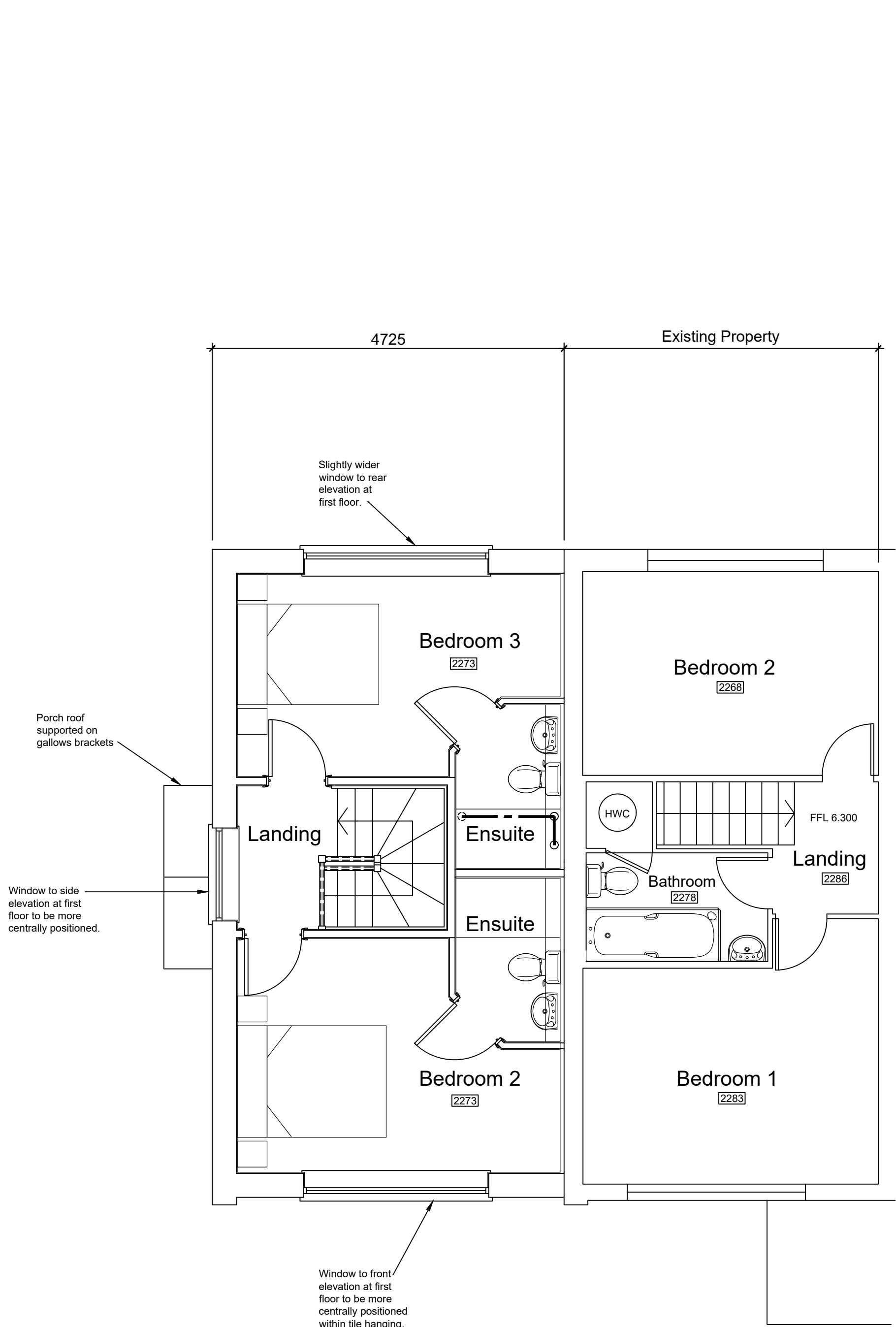
First Floor
