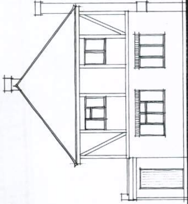
Existing Front (North) Elevation.
