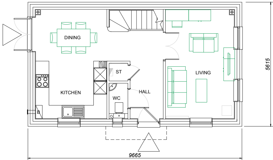
Plot 92 310 GROUND FLOOR PLAN
