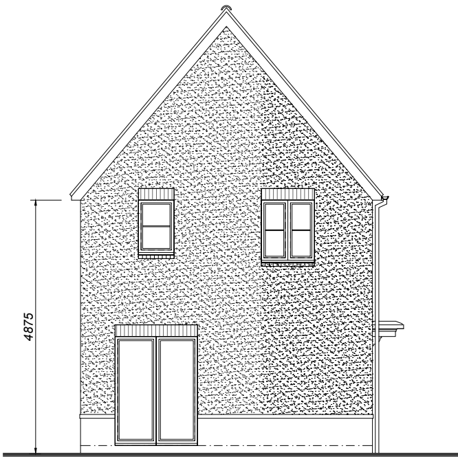
SIDE ELEVATION
