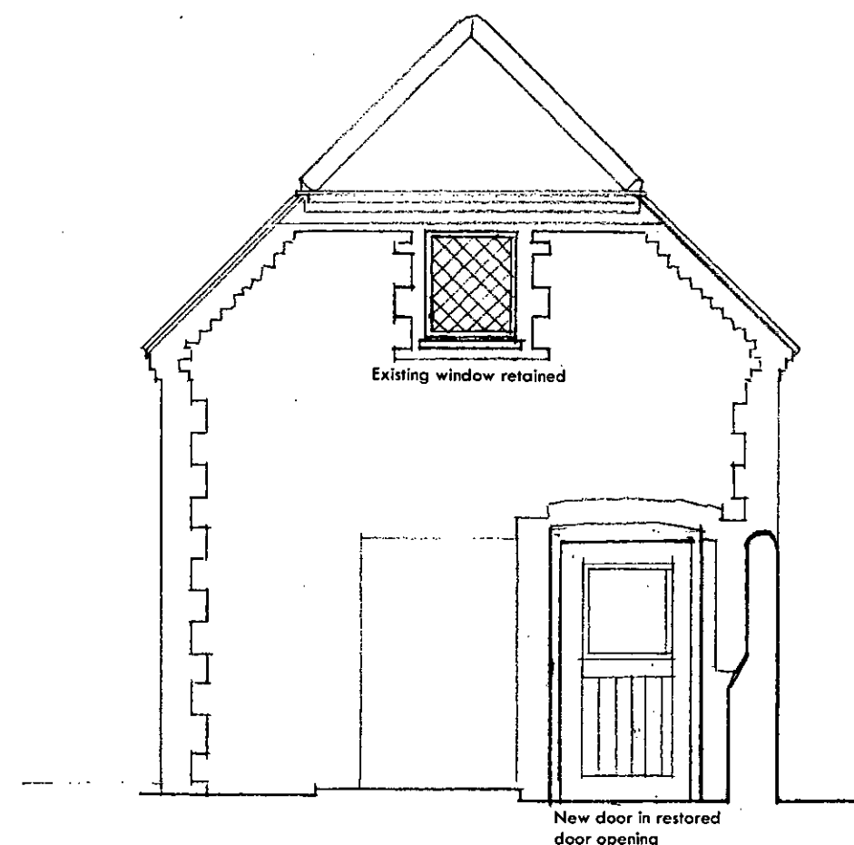
EAST ELEVATION
