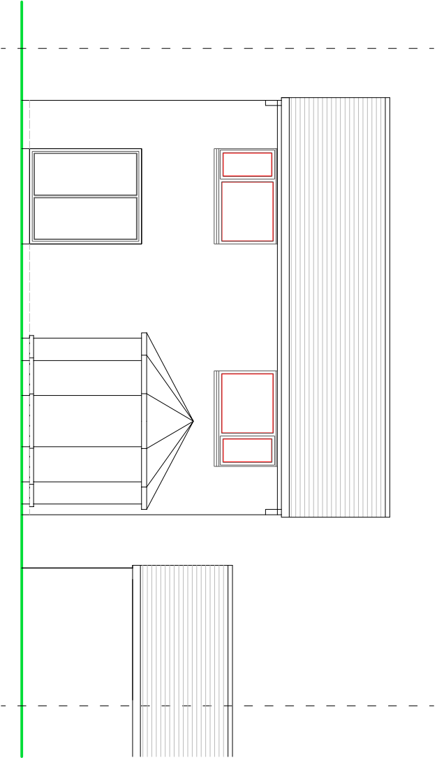
REAR ELEVATION
